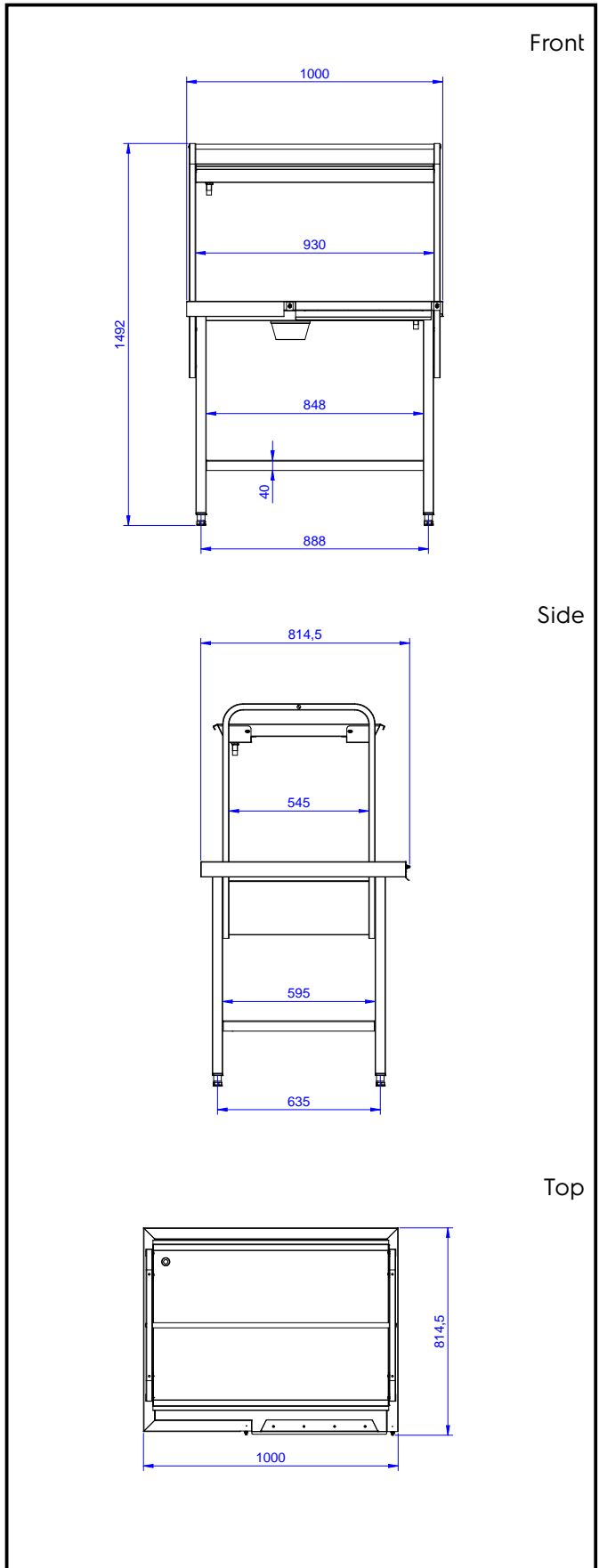
Handling System Sorting Table Left to Right, 1000x800mm
